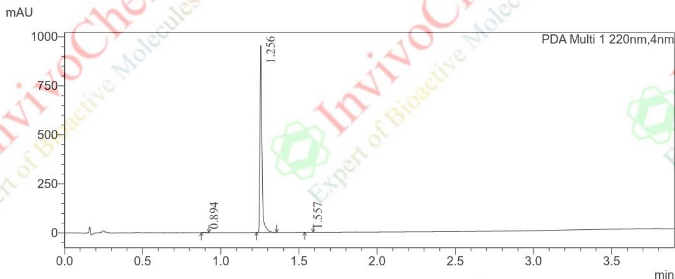
Peak Table PDA Ch1 220nm
