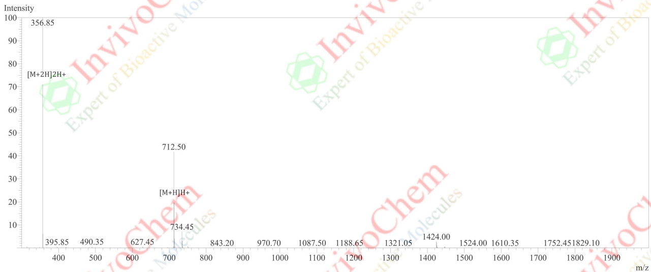
MS Spectrum
