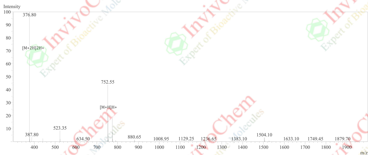
MS Spectrum
