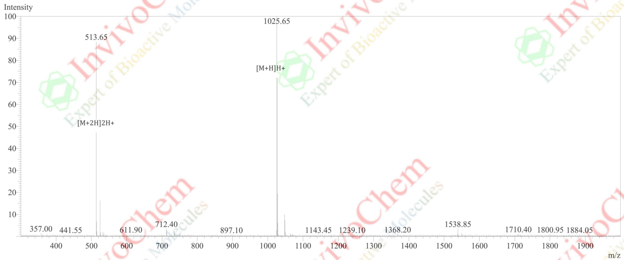
MS Spectrum
