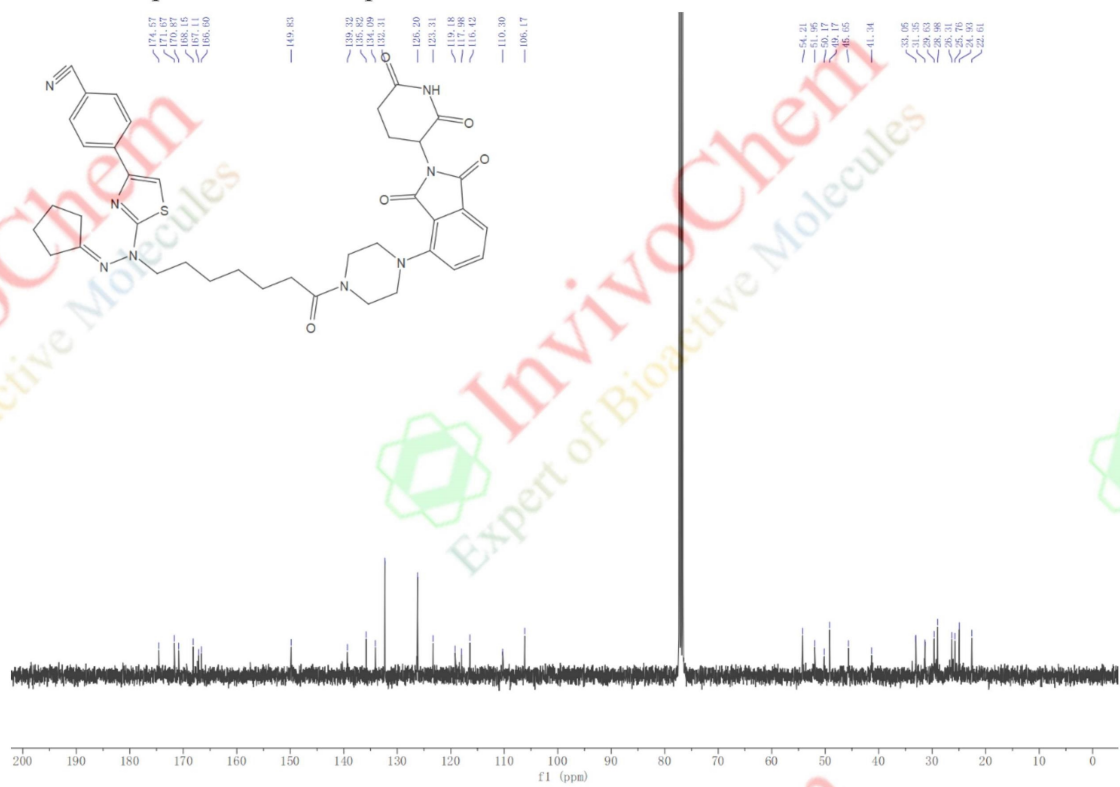
13 C NMR Spectrum for compound 1192.
